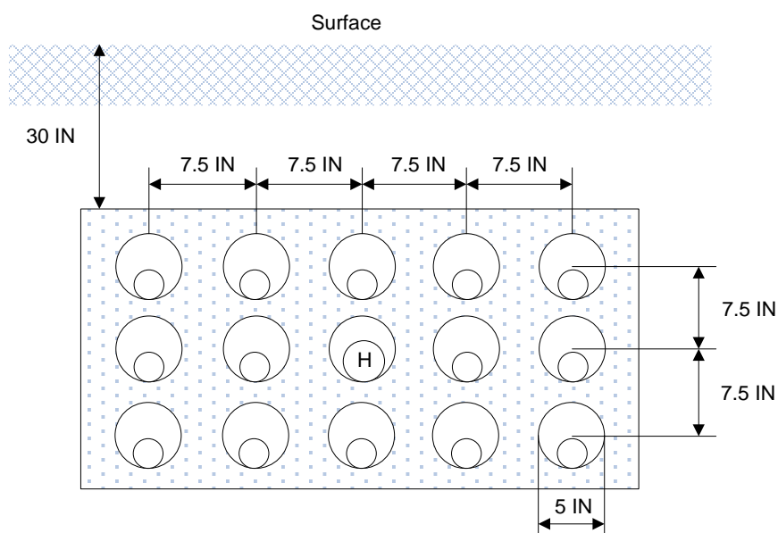
Figure 1. 3 × 5 duct bank arrangement
